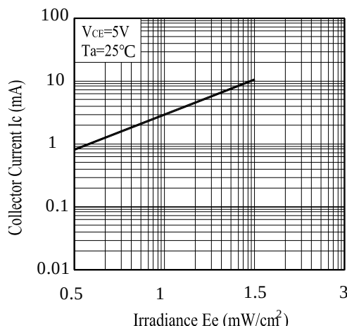
Fig.6 Collector Current vs.
